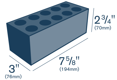
horizontal coursing 3/8" mortar joint
